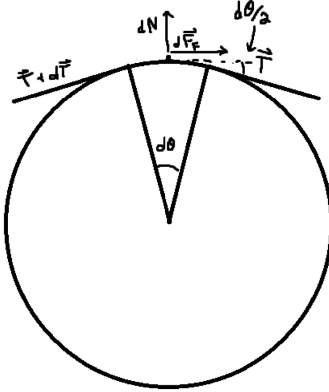
Figure 27: Free-body diagram of a differential belt element spanning d\theta .
